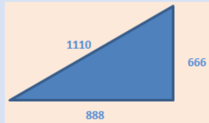
Pythagorean triangle of the proportion 3:4:5
